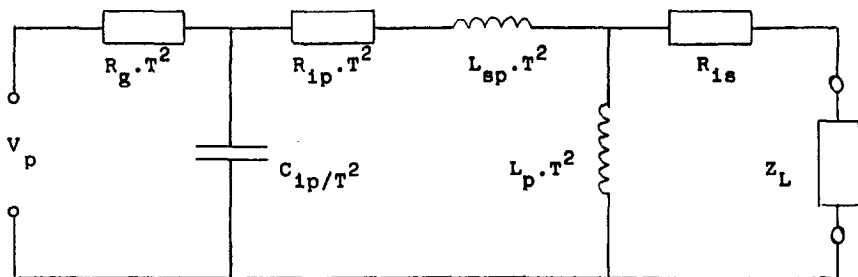
Figure 1-3: Equivalent Circuit Step-Down Output Transformer
