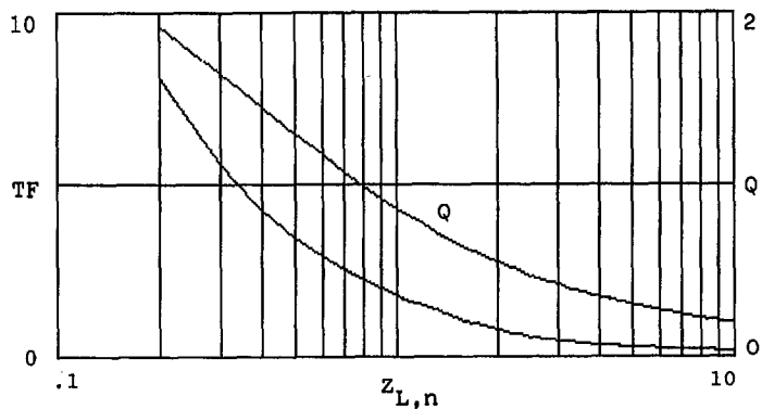
FIGURE 4-5: Tuning Factor as function of normalized load ( \alpha = 1 , \beta = 3 when Z_L = 1 \Omega ) (balanced Triode mode)
