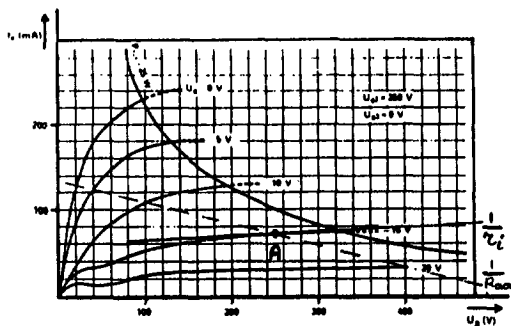
FIGURE 1-1: EL34 Characteristics
