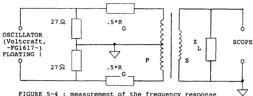
FIGURE 5-4 : measurement of the frequency response
