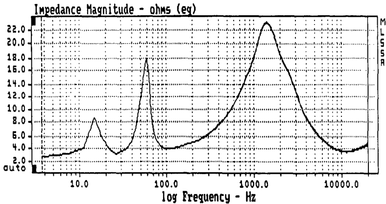
FIGURE 5-2: example of measured impedance of a loudspeaker
