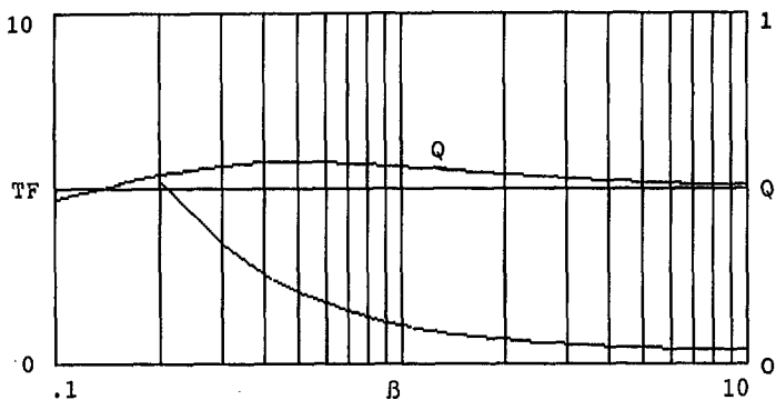
FIGURE 4-1: Tuning Factor (left hand scale) and Q-factor (right hand scale) for \alpha = .5
